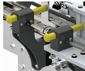
Maintenance-free, robust rack and pinion adjusters
