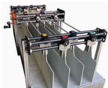
Easily create multiple lanes for different applications or products. Rapidly move unused lane dividers to conveyor outer edge when not in use.
